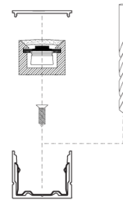
DL-AC-FLEX2-JA8-MC Plastic Mounting Clip
