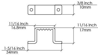
DL-AC-FLEX2-JA8-MC-HW Hardwire clips required 2 per section
