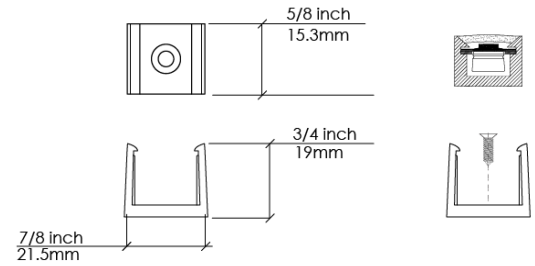
DL-AC-FLEX2-JA8-MC Plastic Mounting Clip
