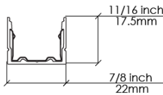
DL-AC-FLEX2-JA8-CH6M18 6 Feet Metal Channel
