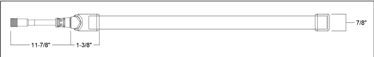
DL-FLEX2-LNSB with DL-FLEX2-LNSB-ES-PC-M and DL-FLEX2-LNSB-EC
