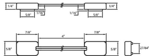
MMT-CCE04 Connecting Cable - wire from the end
