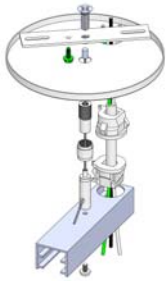
H1CS048P ■ ■ ■ Cable Suspension w/ Powerfeed
